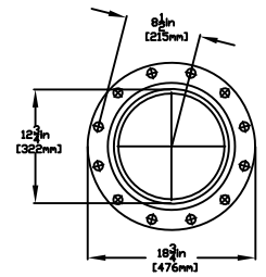
FLANGE DETAIL x2
