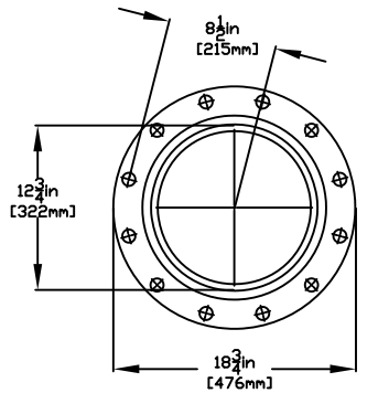
FLANGE DETAIL
