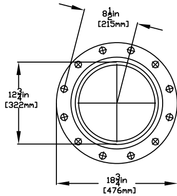
FLANGE DETAIL
